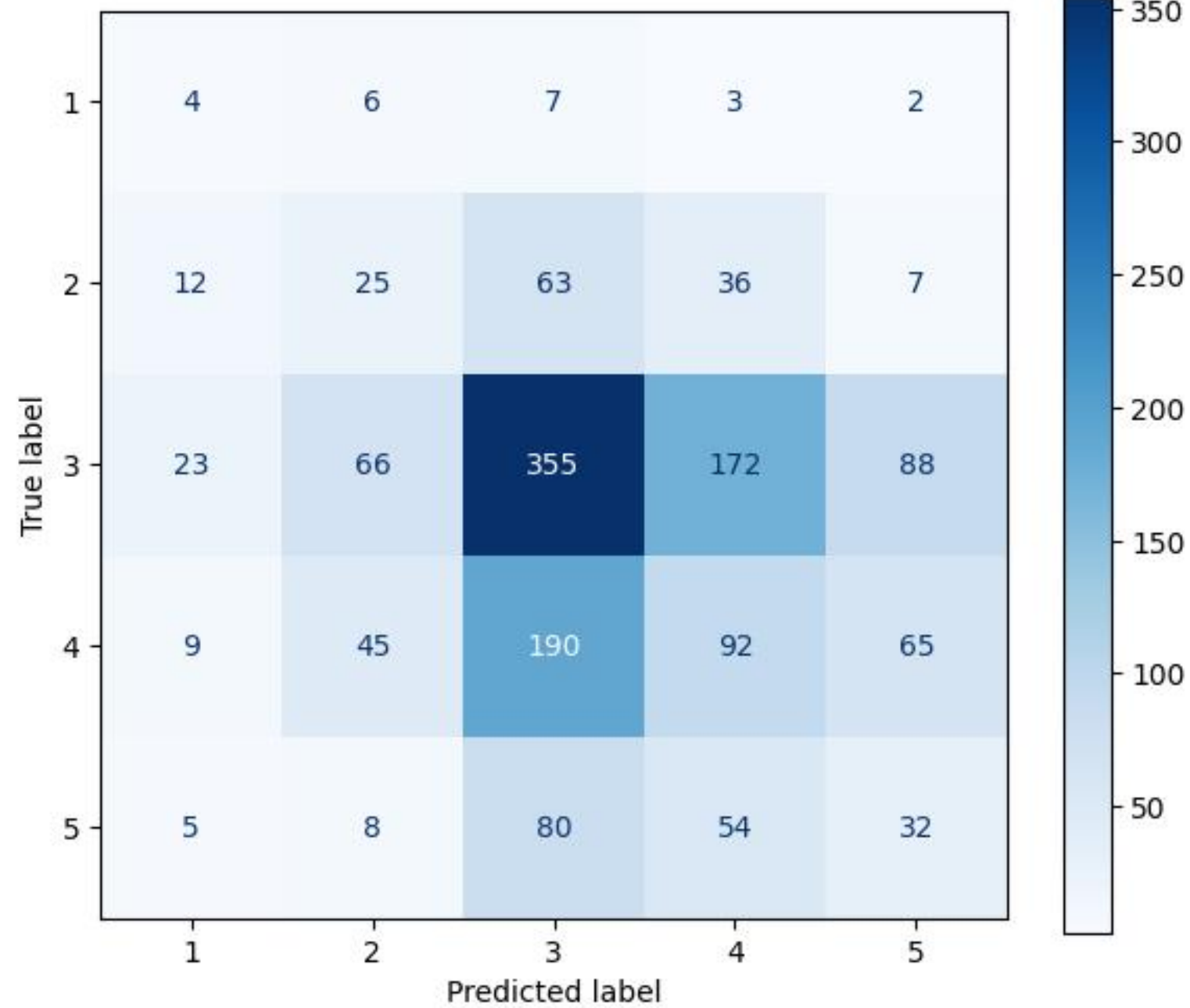
Best Model: CV Confusion Matrix
