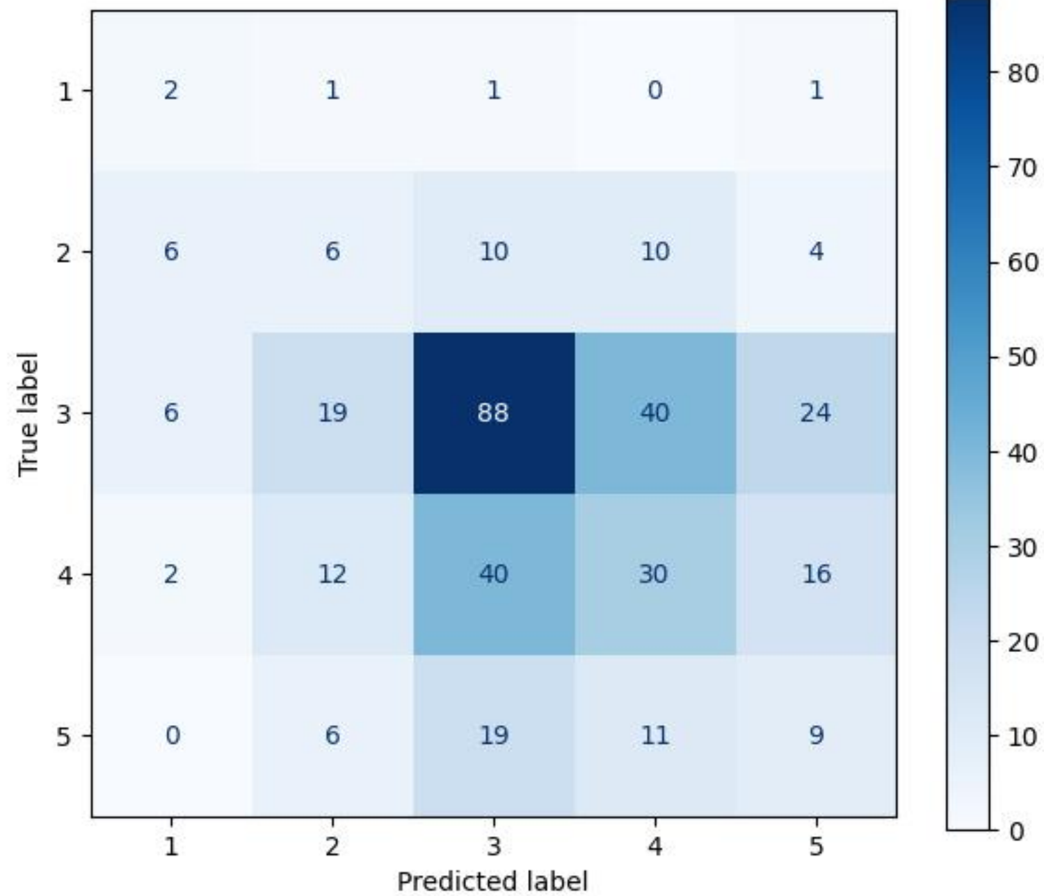
Best Model: Test Confusion Matrix
